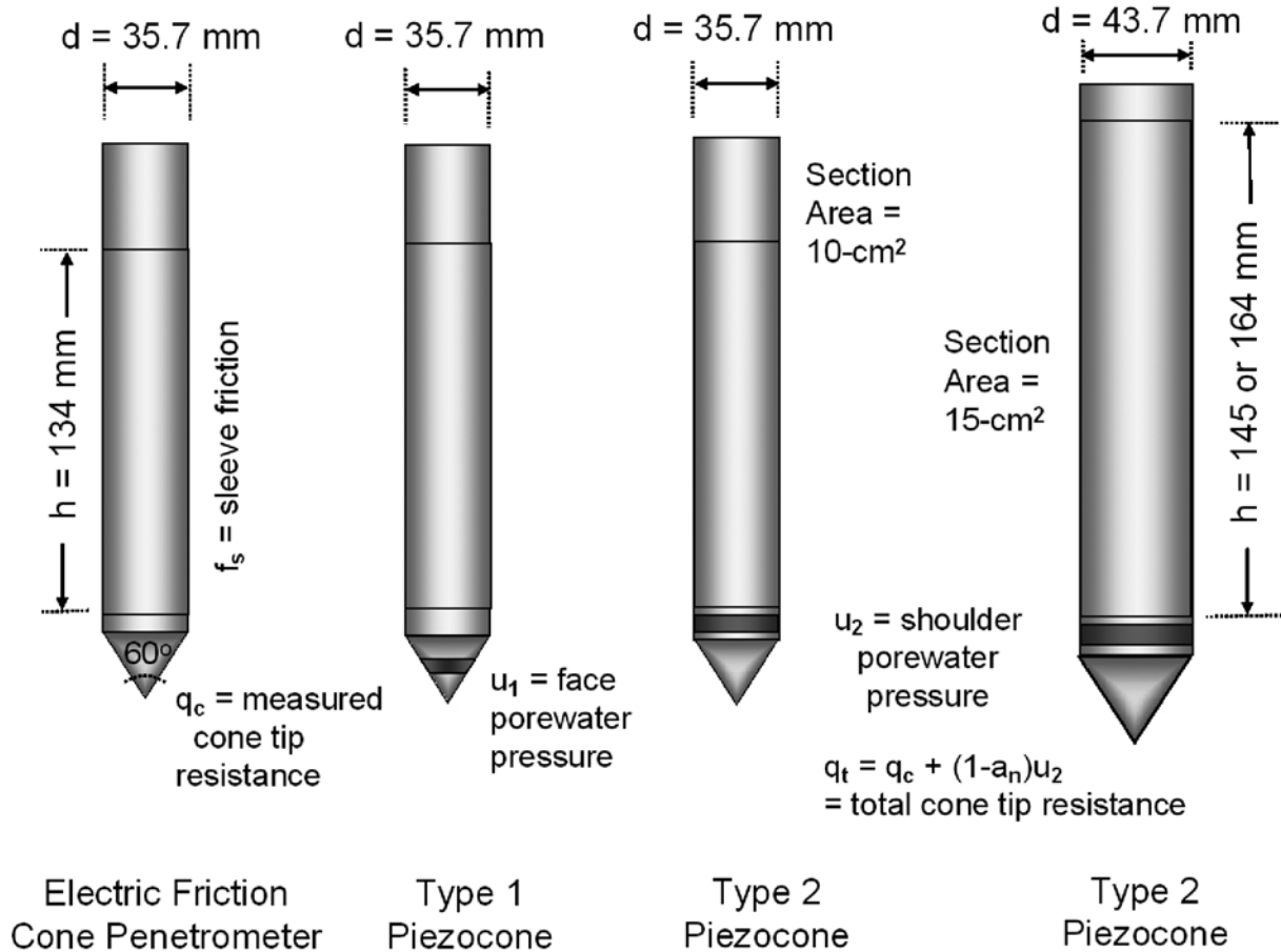
FIG. 3 Penetrometer Design Configurations: (a) Electric Friction-type, (b) Type 1 Piezocone, (c) Standard 10-cm 2 Type 2 Piezocone, and (d) 15-cm 2 Type 2 Version (7)
