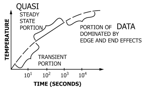
(A) IDEALIZED CURVE
